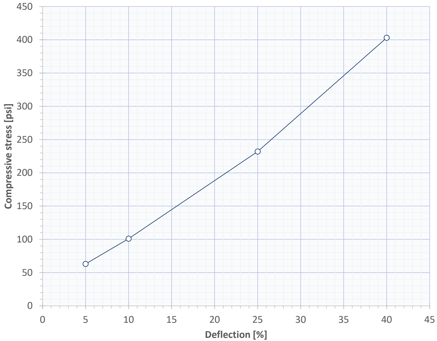
Compression-Deflection Data for SSP502F-60
