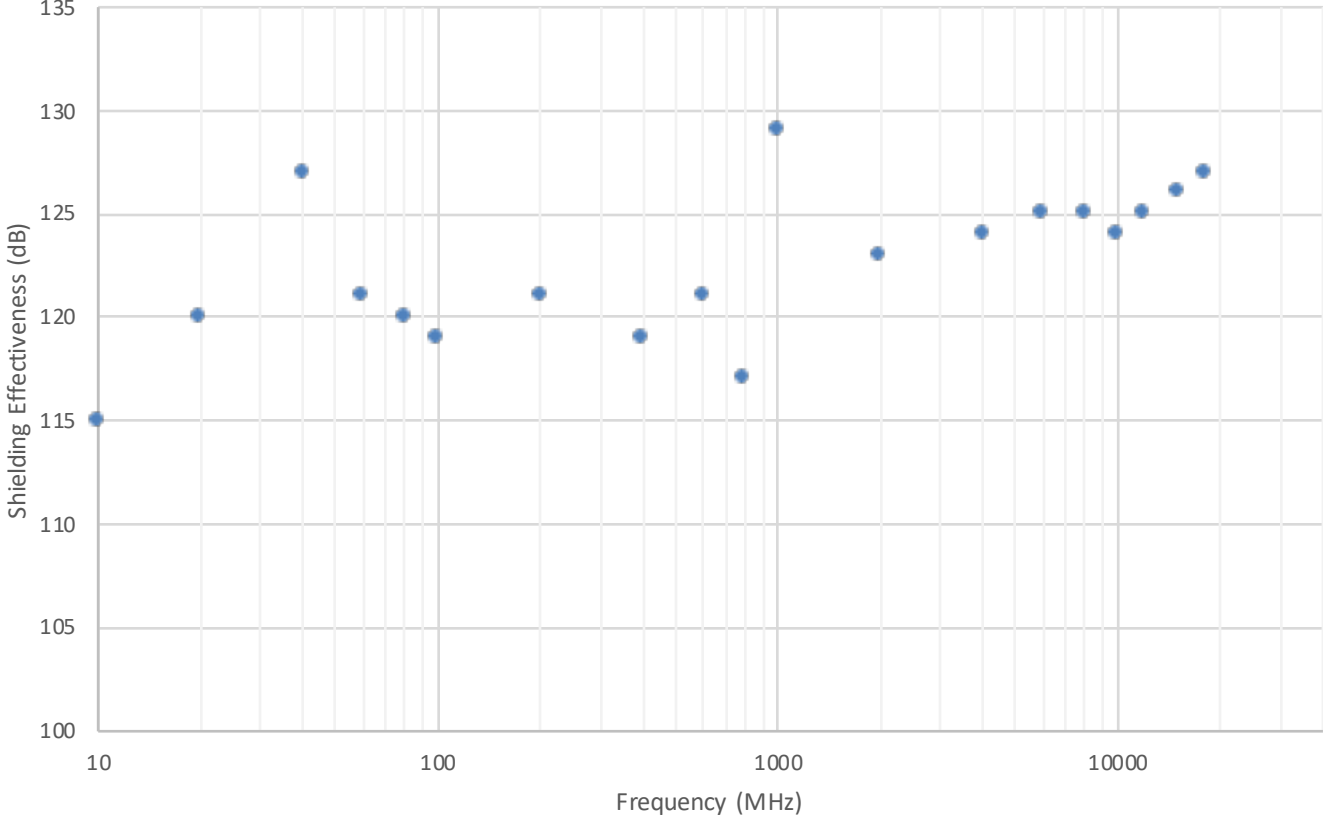
Shielding Effectiveness (dB) - SSP502-60V0 (DF036)
